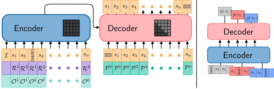
Figure 2: COFS Overview. (Left): We use a BART-like encoder-decoder model, with bidirectional attention in the encoder and an autoregressive decoder. The encoder encodes the layout as a set without ordering information and therefore does not receive ( absolute ) position tokens. However, to disambiguate a single object, the encoder receives additional information in the form of Relative Position Tokens \mathcal{R}^i , and the Object Index Tokens \mathcal{O}^i . During training, object order is randomly permuted and a random proportion of tokens is replaced with a [MASK] token. The decoder outputs a sequence representation of the set and is trained with Absolute Position Tokens \mathcal{P}^i . It performs two tasks - 1. copy-paste: the decoder copies the unmasked attributes to their proper location 2. mask-prediction: the decoder predicts the actual value of the token corresponding to a [MASK] token in the encoder input. (Right): During inference, we measure the likelihood of a given test set token using an input sequence where only this token is masked out.
