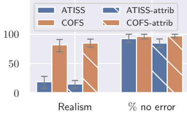
Figure 3: Perceptual Study. We compare the percentage of comparisons in which users found either method more realistic (left), and in which users did not find any obvious errors such as object intersections (right), with 95% confidence intervals as error bars. Results show a large advantage for COFS in realism of layouts generated with attribute-level conditioning (-attrib), and a smaller, but still significant advantage in the percentage of error-free layouts. This advantage is also present in the unconditional setting.
